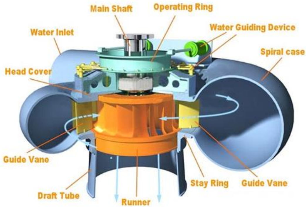
Francis Turbine
