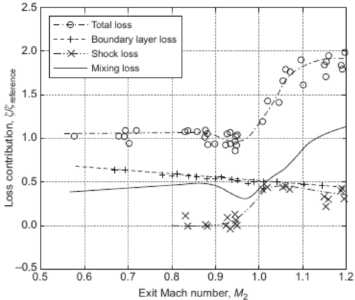
Variation of loss coefficient with Mach number for a turbine cascade at a Reynolds number of 1 3 106.
