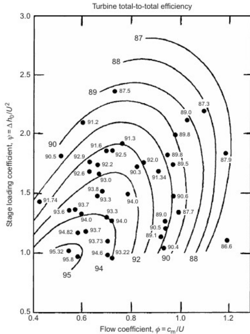
Smith chart for turbine stage efficiency.
