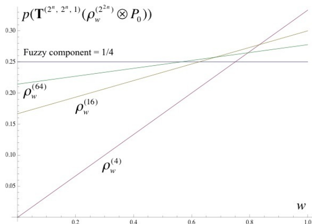
Fig. 1. Fuzzy component vs. incidence of \text{tr}(\mathbb{T}_p^{(2^n, 2^n, 1)}(\mathbf{M}(\rho_w^{(2^{2n})}) \otimes P_0)) .
